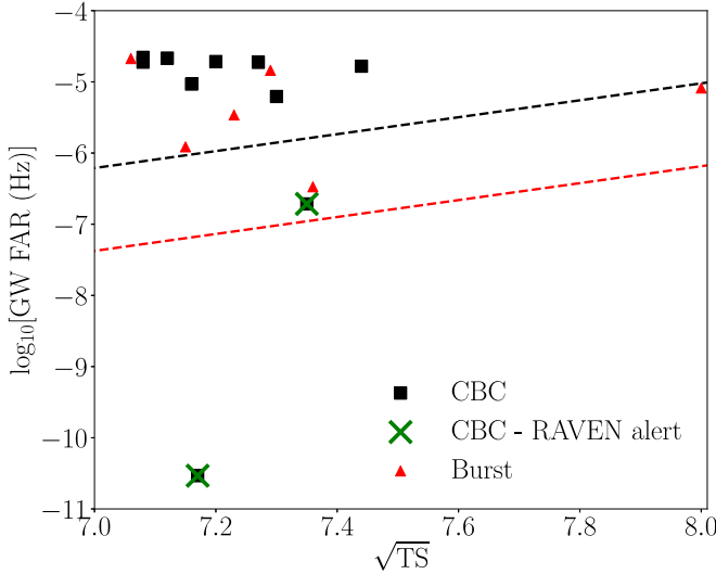
Figure 6. Distribution in the GW FAR– \sqrt{\text{TS}} plane of all the triggers that passed the threshold \text{FAR}_{\text{GRB}} < 10^{-3} Hz. Triggers in the regions below the black and red dashed lines (marked with a green cross) would have triggered the RAVEN alert system, for CBC and Burst events, respectively. The plot does not include all the triggers that have a \sqrt{\text{TS}} > 8 which turned out to be spurious artifacts.
