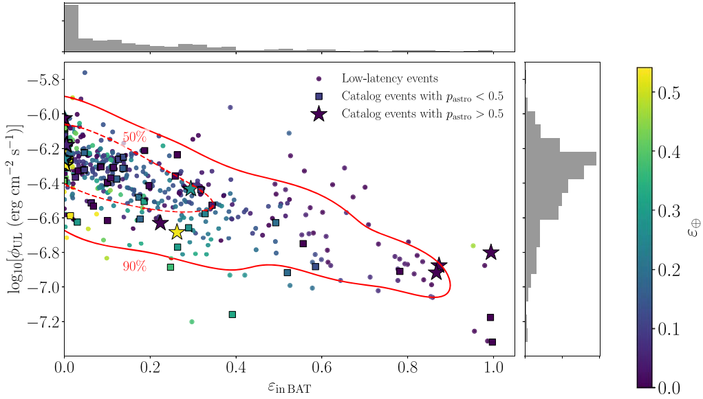
Figure 4. The 15–350 keV flux upper limit \phi_{UL} derived with NITRATES as a function of \epsilon_{in\ BAT} , namely the probability that the GW candidate is contained inside the BAT FOV. The plot includes all the GW candidates received during O3, including both Burst and CBC events. With different symbols, we distinguish the GW candidates received in low latency and the ones confirmed and included in the O3 catalog, separated in p_{astro} > 0.5 and p_{astro} < 0.5 . The dashed and solid red lines are the 50% and 90% containment regions of the scatter plot, respectively. The one-dimensional histograms of \phi_{UL} and \epsilon_{in\ BAT} are reported on the sides. The color bar indicates the value of \epsilon_{\oplus} , the probability that the GW candidate is occulted by the Earth.
