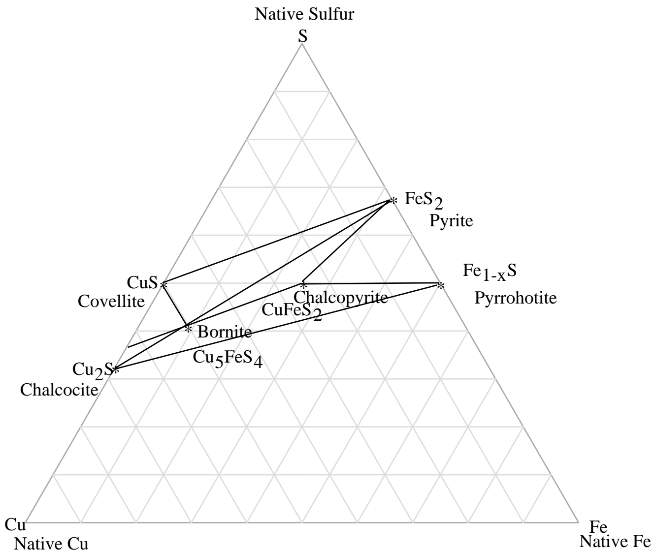
Figure 1.1 Some sulfides
